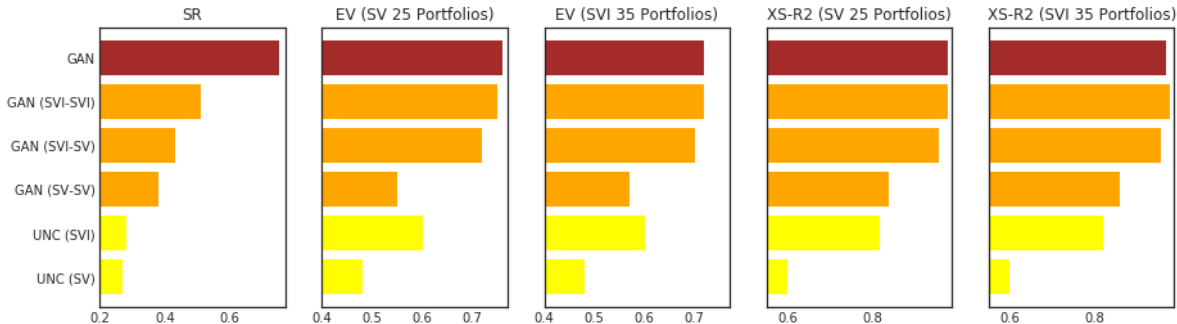
Figure 4: GAN Illustration
