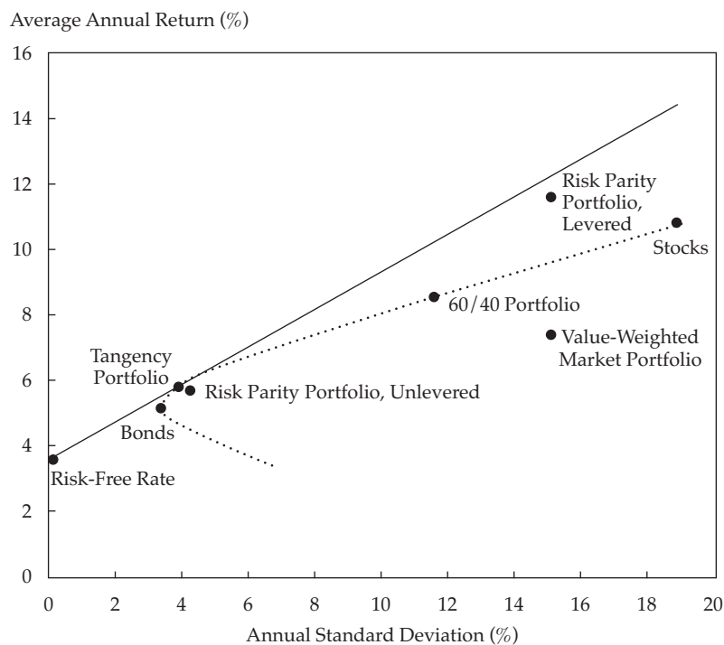
Figure 2. Efficient Frontier, 1926–2010
