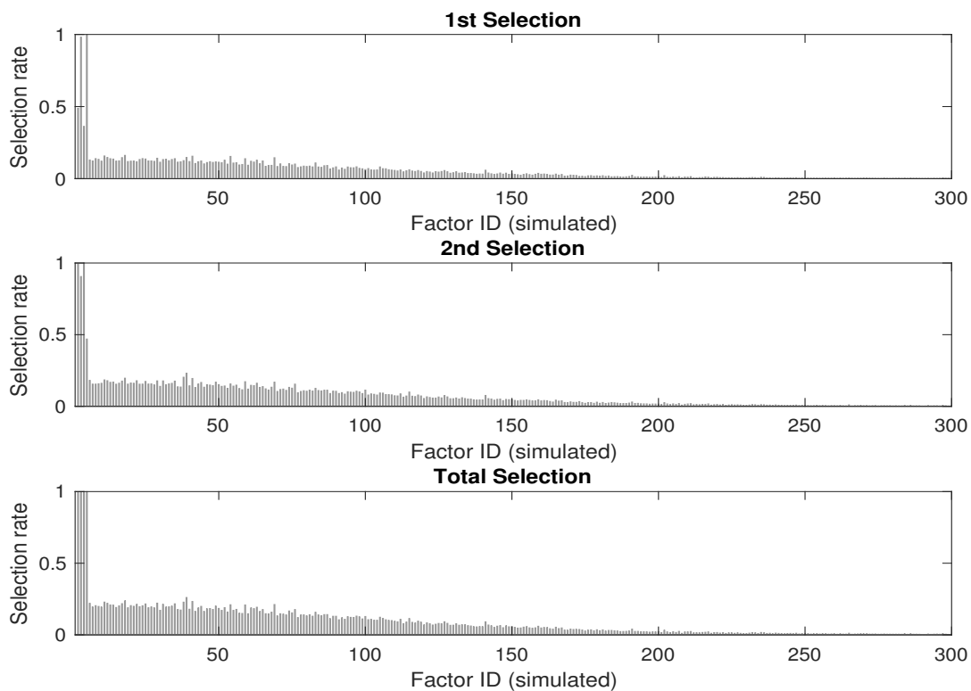
Figure 2: Histograms of the Selected Variables
